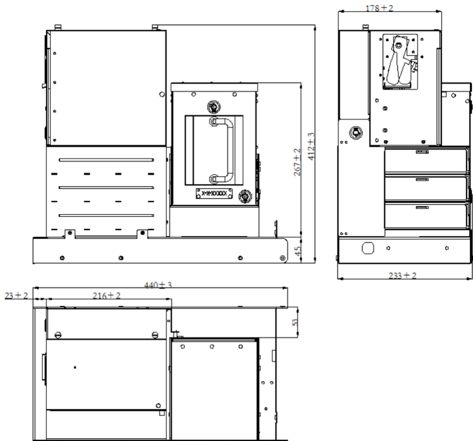
Figure 2 Module dimension
